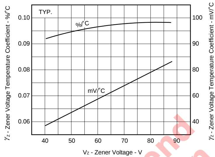
Figure 5. \gamma_z vs. V_z Example of Characteristics
