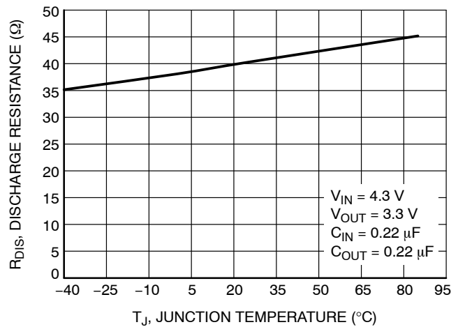
Figure 24. Discharge Resistance vs. Temperature
