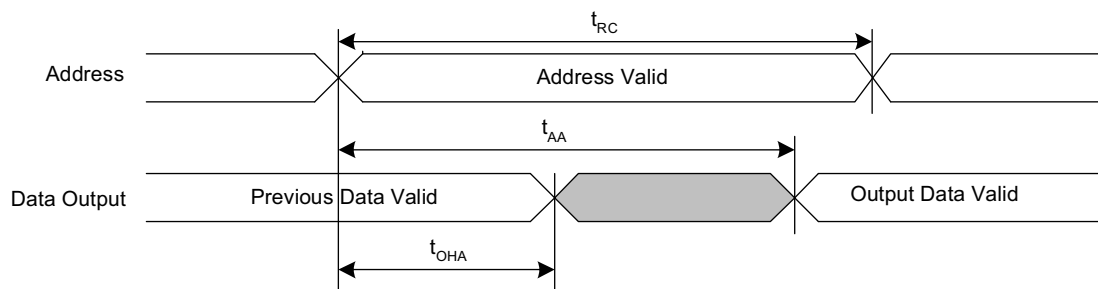
Figure 5. SRAM Read Cycle #1: Address Controlled [11, 12, 15]
