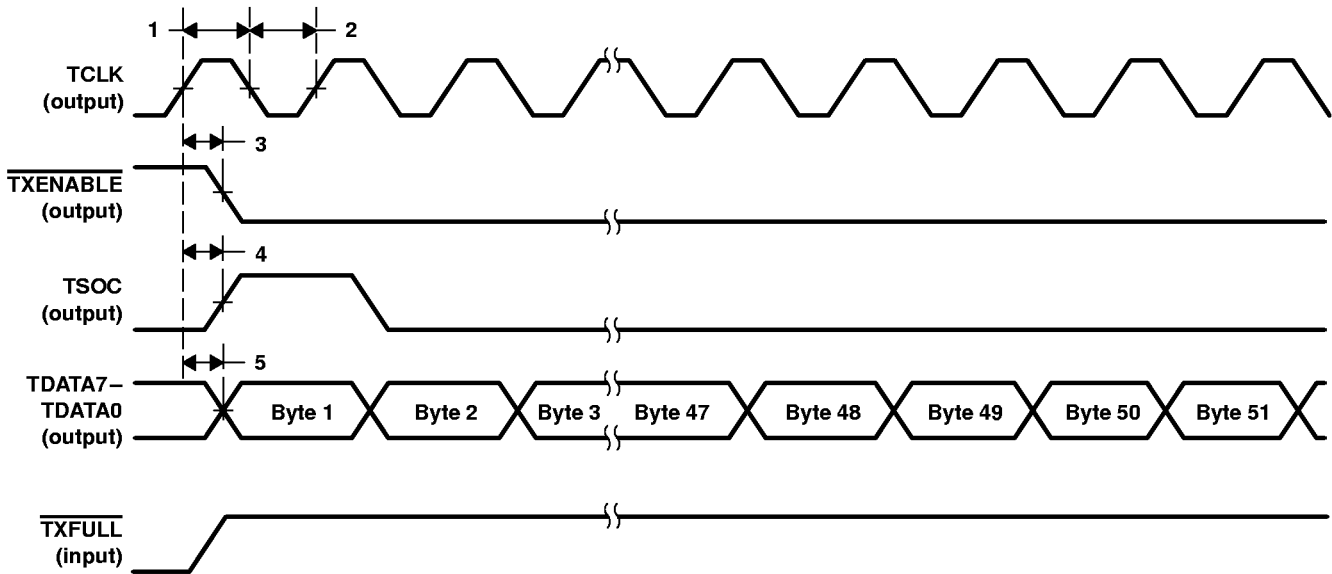
Figure 2. Transmit-Cell Interface
