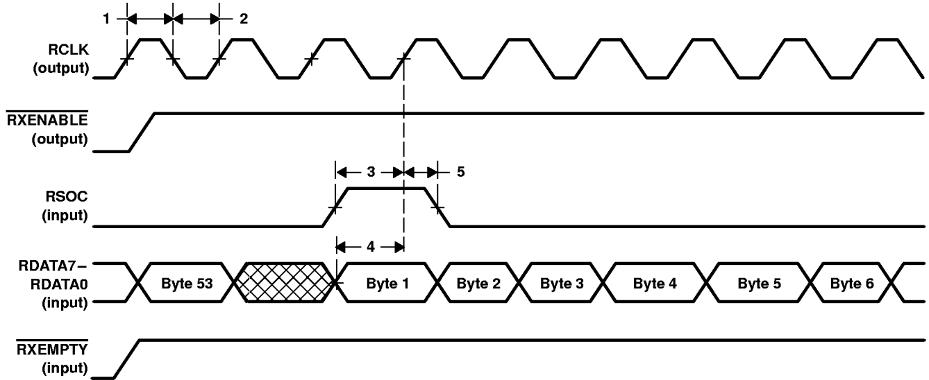
Figure 1. Receive-Cell Interface
