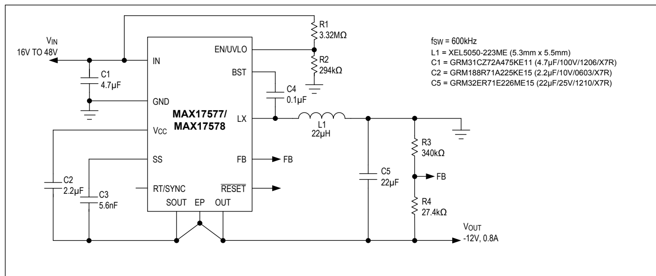
Figure 7. MAX17577 and MAX17578 -12V Output Application Circuit Compatible with 24V Input Bus Voltage
