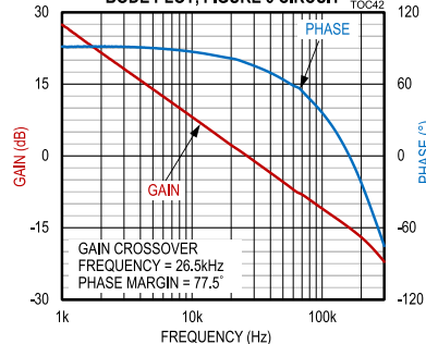
MAX17577, -5V OUTPUT, BODE PLOT, FIGURE 6 CIRCUIT
