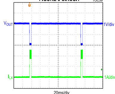
MAX17577/MAX17578, -5V OUTPUT, OVERLOAD PROTECTION FIGURE 5 CIRCUIT
