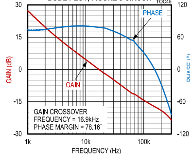
MAX17577, -12V OUTPUT, BODE PLOT, FIGURE 8 CIRCUIT
