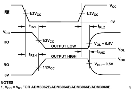
Figure 8. Receiver Enable and Disable Timing Diagram
