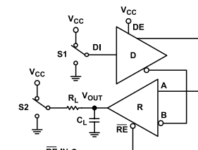
Figure 43. Receiver Enable/Disable from Shutdown
