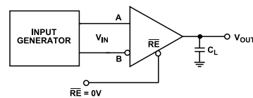
Figure 42. Receiver Propagation Delay/Skew
