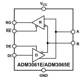
Figure 1. ADM3061E/ADM3065E Functional Block Diagram
