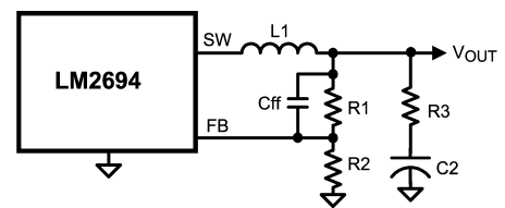
FIGURE 17. Low Output Ripple Using a Feedforward Capacitor
