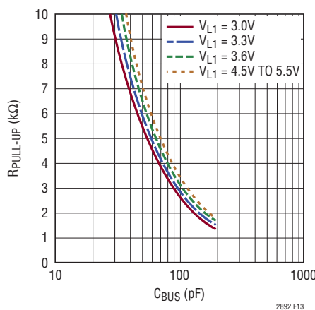
Figure 13. Maximum Fast Speed Pull-Up Resistance on SDA1
