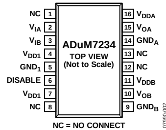
Figure 2. Pin Configuration
