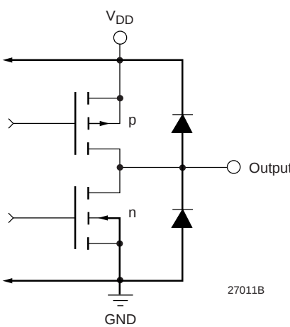
Figure 4. Equivalent Digital Output Circuit
