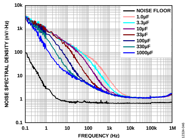
Figure 2. Noise Spectral Density for Different Values of C_{\text{BY}}
