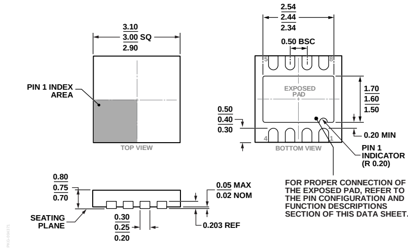
Figure 65. 8-Lead Lead Frame Chip Scale Package [LFCSP_WD] 3 mm × 3 mm Body, Very Very Thin, Dual Lead (CP-8-21)
