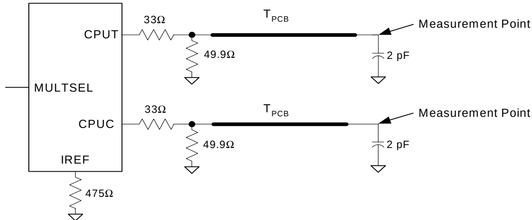
Figure 8. 0.7V Configuration
