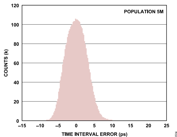
Figure 26. Time Interval Error (TIE) Histogram for D_{OUT1\pm} at 1.25 GHz
