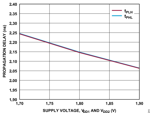
Figure 13. Propagation Delay vs. Supply Voltage, V_{DD1} and V_{DD2}
