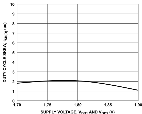
Figure 19. Duty Cycle Skew, t_{SK(D)} vs. Supply Voltage, V_{DD1} and V_{DD2}
