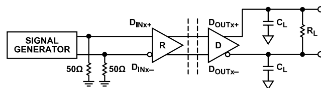
Figure 30. Voltage Definitions
