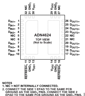
Figure 5. Pin Configuration, LFCSP
