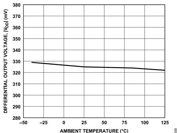
Figure 10. Differential Output Voltage, |V_{OD}| vs. Ambient Temperature
