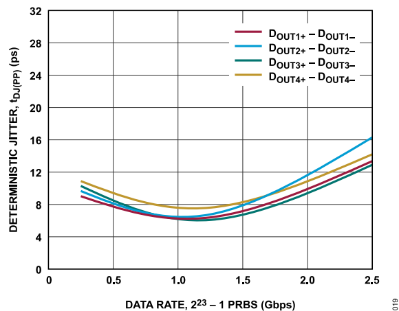
Figure 21. Deterministic Jitter, t_{DJ(PP)} vs. Data Rate, 2^{23} - 1 PRBS
