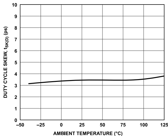
Figure 20. Duty Cycle Skew, t_{SK(D)} vs. Ambient Temperature
