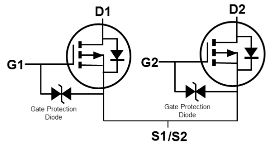
Internal Schematic
