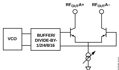
Figure 22. Output Stage
