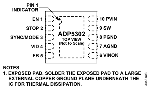
Figure 3. Pin Configuration
