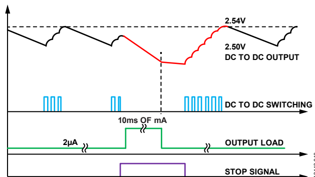
Figure 40. STOP Switching Operation Status
