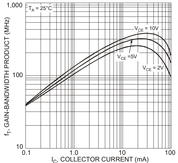
Fig. 7 Typical Gain-Bandwidth Product vs. Collector Current (BC847B Type)
