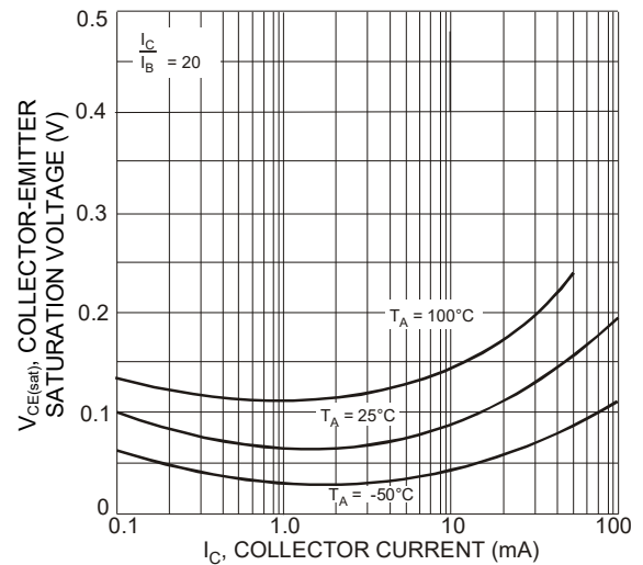
Fig. 5 Typical Collector-Emitter Saturation Voltage vs. Collector Current (BC847B Type)
