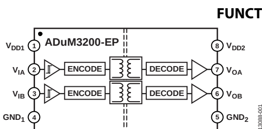
Figure 1. ADuM3200-EP Functional Block Diagram
