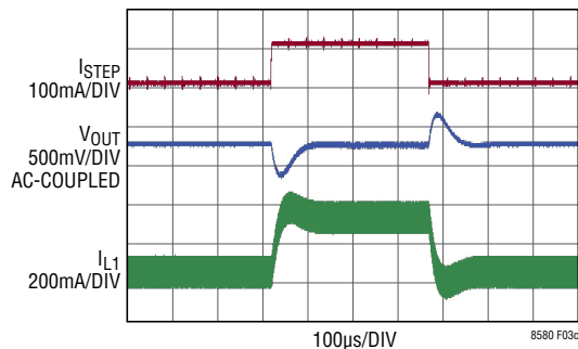
(3c) Transient Response Is Well Damped
