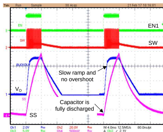
Figure 18. Passive Discharge With 2-MΩ Resistor
