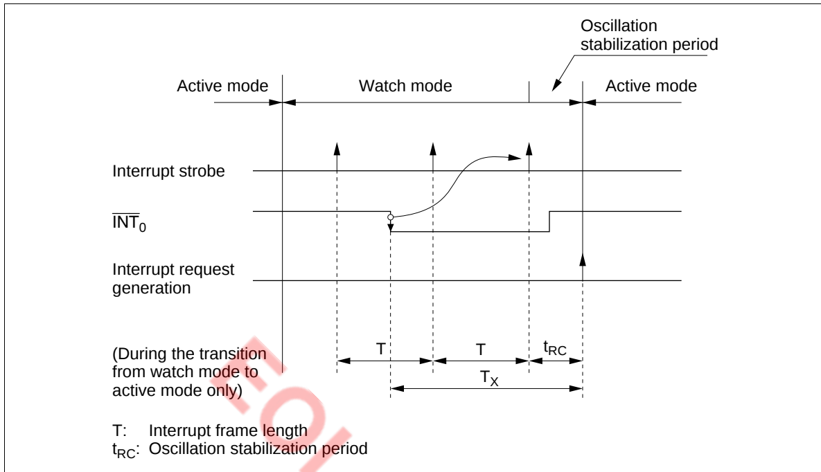
Figure 12 Interrupt Frame
