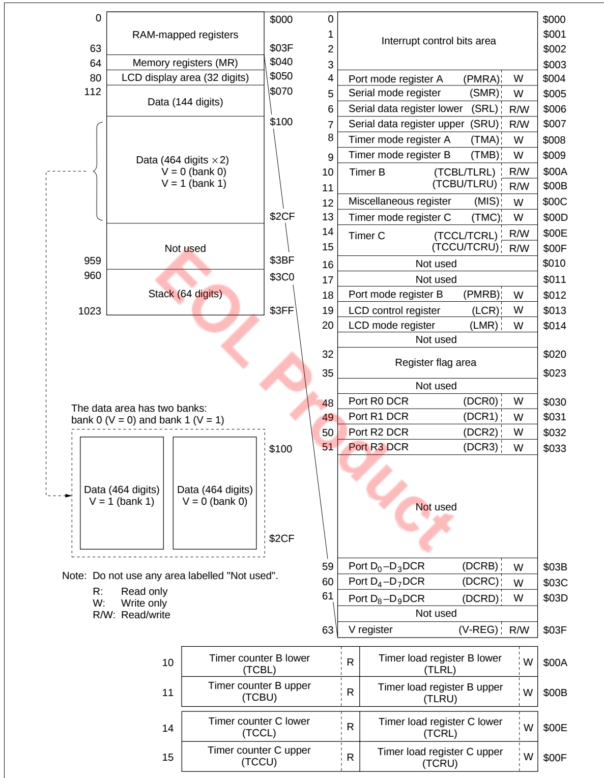
Figure 2 RAM Memory Map (1,184-digit × 4-bit)
