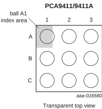
Fig 2. Pin configuration WLCSP9 package
