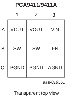
Fig 3. Ball mapping for WLCSP9
