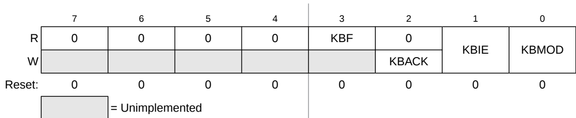
Figure 7-3. KBIX Status and Control Register
