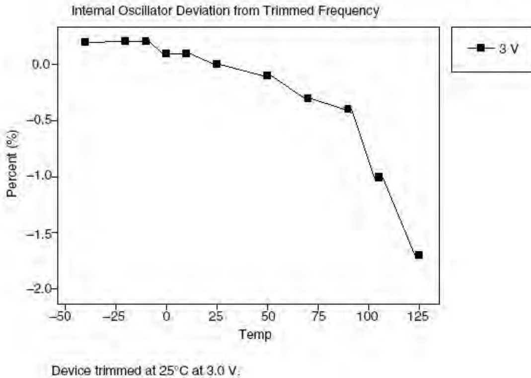
Figure A-11. Internal Oscillator Deviation from Trimmed Frequency
