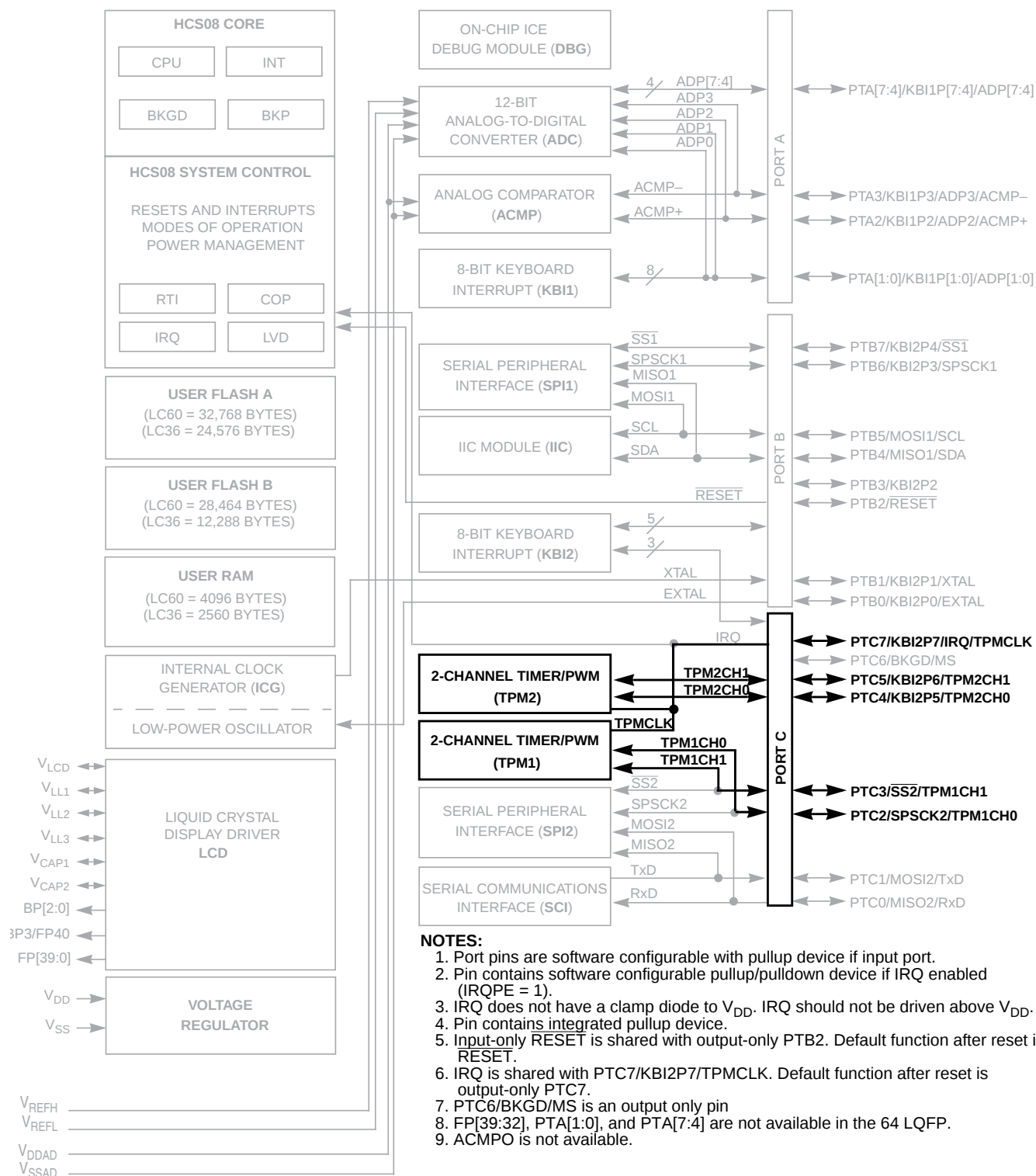
Figure 11-1. MC9S08LC60 Series Block Diagram Highlighting TPM Block and Pins
