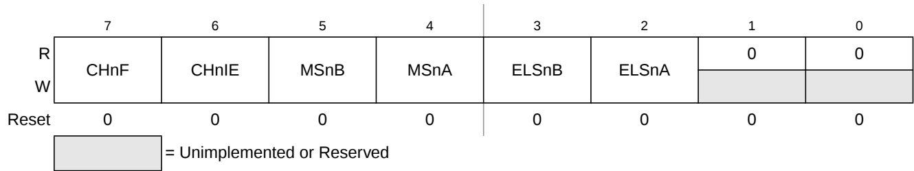
Figure 11-8. Timer x Channel n Status and Control Register (TPMxCnSC)
