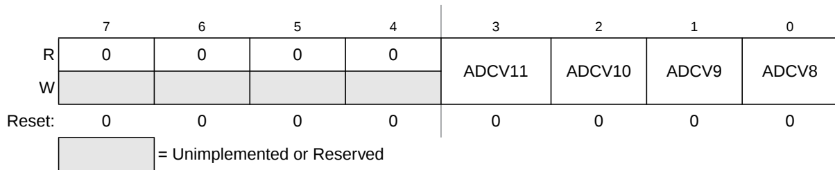
Figure 15-8. Compare Value High Register (ADCCVH)
