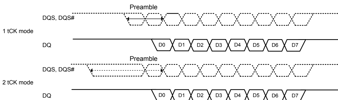
Figure 78. 1 t_{CK} vs. 2 t_{CK} WRITE Preamble Mode
