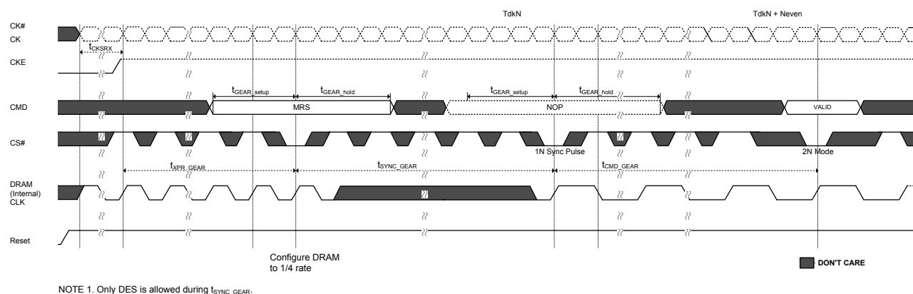
Figure 39. Gear down (2N) mode entry sequence during initialization
