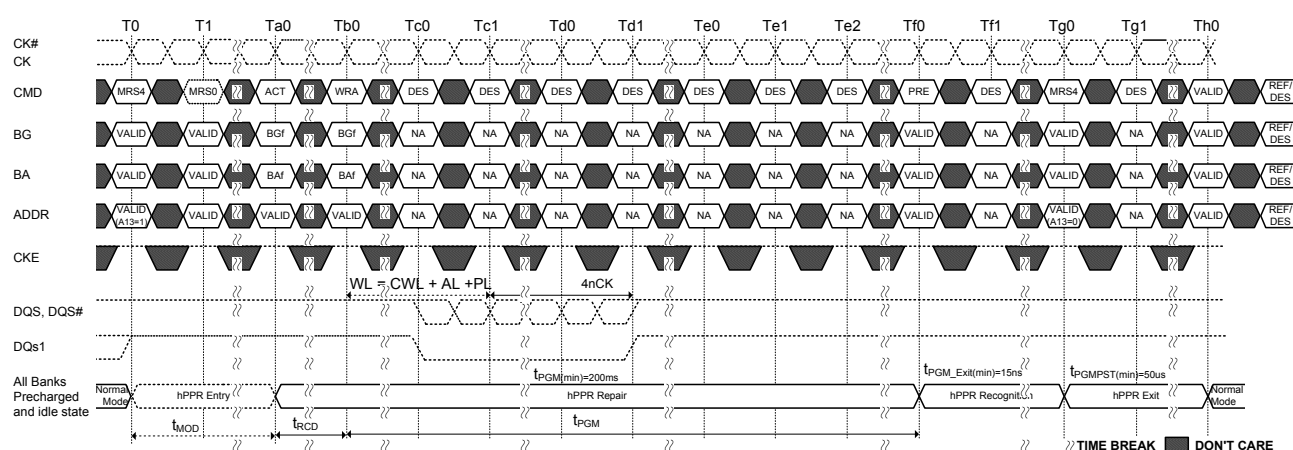
Figure 160. Hard Fail Row Repair (WR Case)
