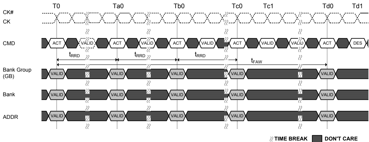
Figure 75. t_FAW Timing
