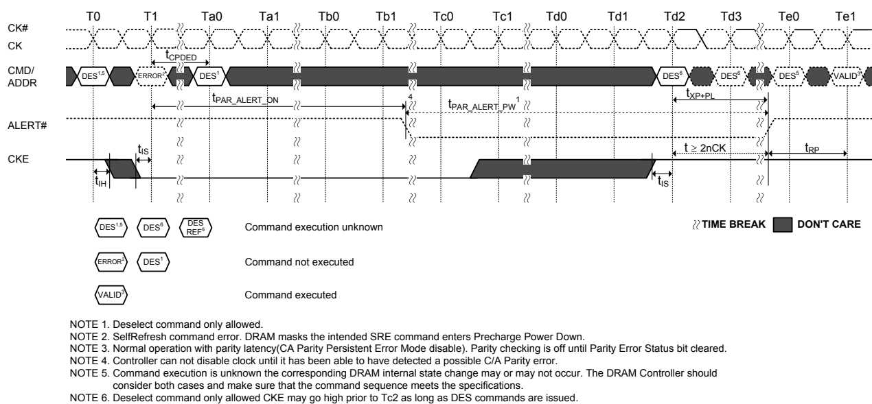
Figure 58. CA Parity Error Checking - SRE Attempt
