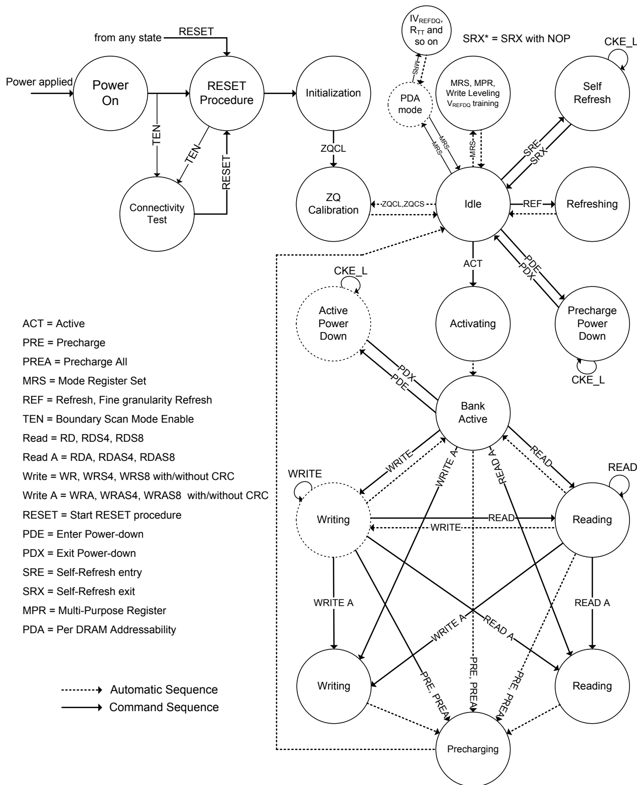
Figure 3. State Diagram
