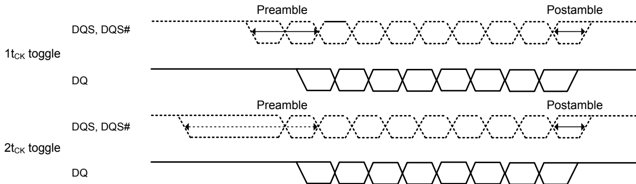
Figure 85. WRITE Postamble
