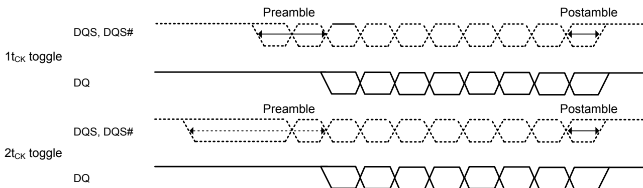
Figure 84. READ Postamble
