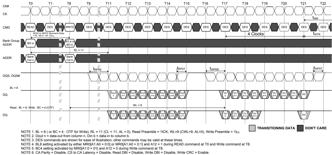
Figure 119. READ (BL8) to WRITE (BL8 or BC4: OTF) with 1t CK Preamble and Write CRC in Same or Different Bank Group
