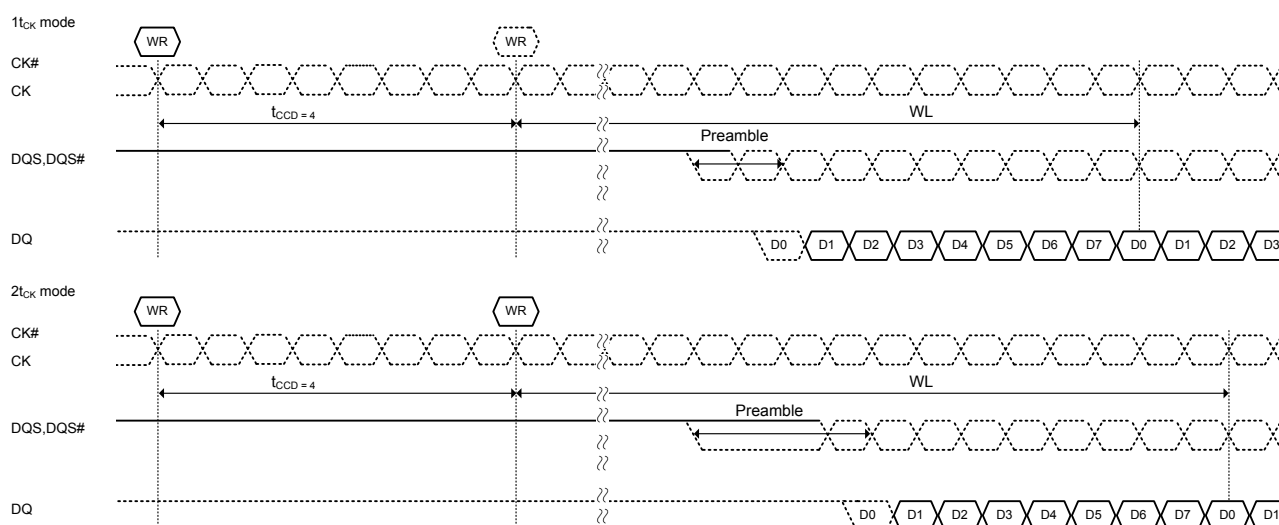
Figure 79. t_{CCD}=4 (AL=PL=0)
