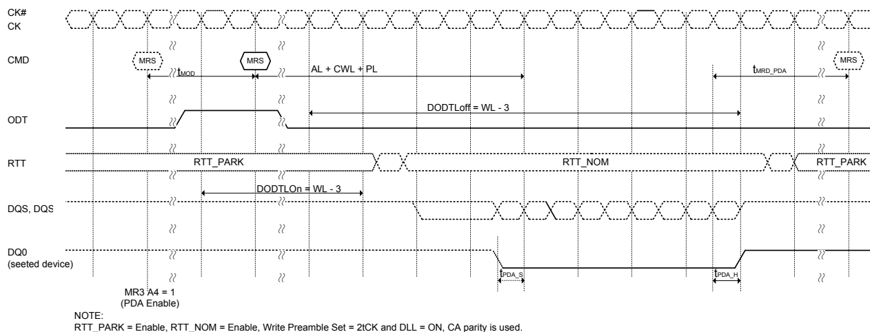
Figure 52. MRS w/ per DRAM addressability (PDA) issuing before MRS
