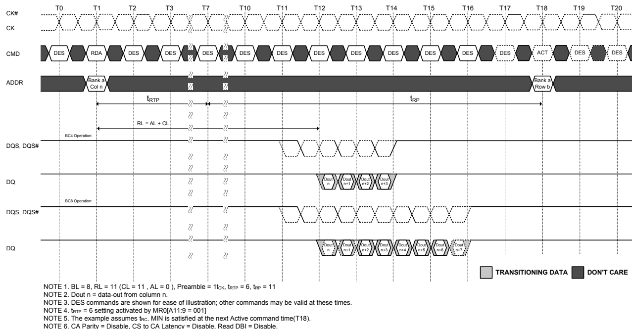
Figure 114. READ with Auto Precharge and 1t_{CK} Preamble
