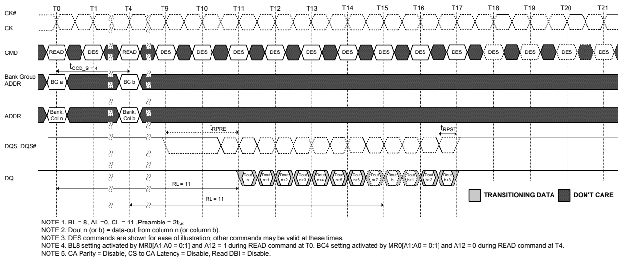
Figure 104. READ (BL8) to READ (BC4) OTF with 2t_{CK} Preamble in Different Bank Group
