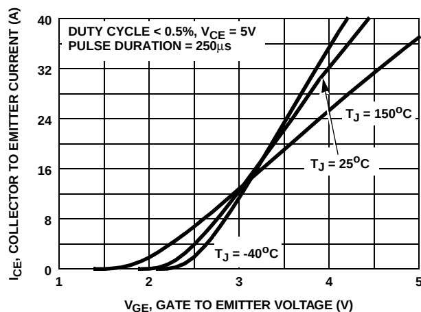
FIGURE 10. TRANSFER CHARACTERISTIC
