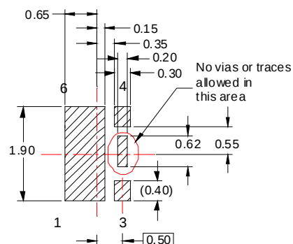
RECOMMENDED LAND PATTERN OPT 2
