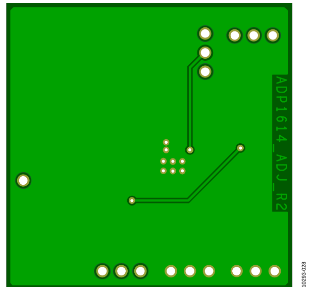
Figure 36. ADP1614 Recommended Bottom Layer Layout for the Adjustable Current-Limit Boost Application
