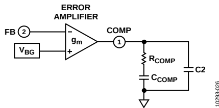
Figure 34. Compensation Components
