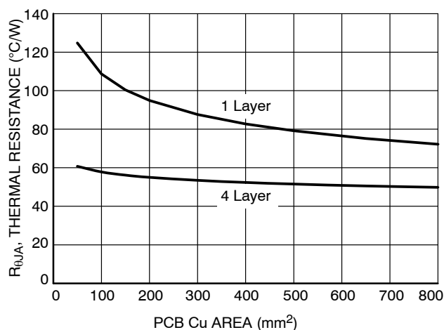
Figure 20. R_{\theta JA} vs. PCB CU Area (SOIC-8 EP Package)
