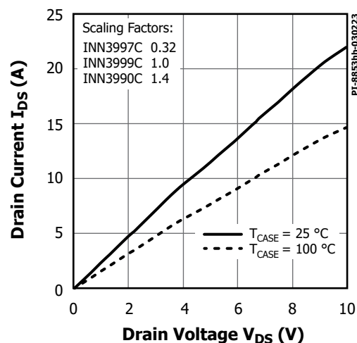
Figure 39. Output Characteristics.
