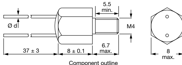
Component outline
