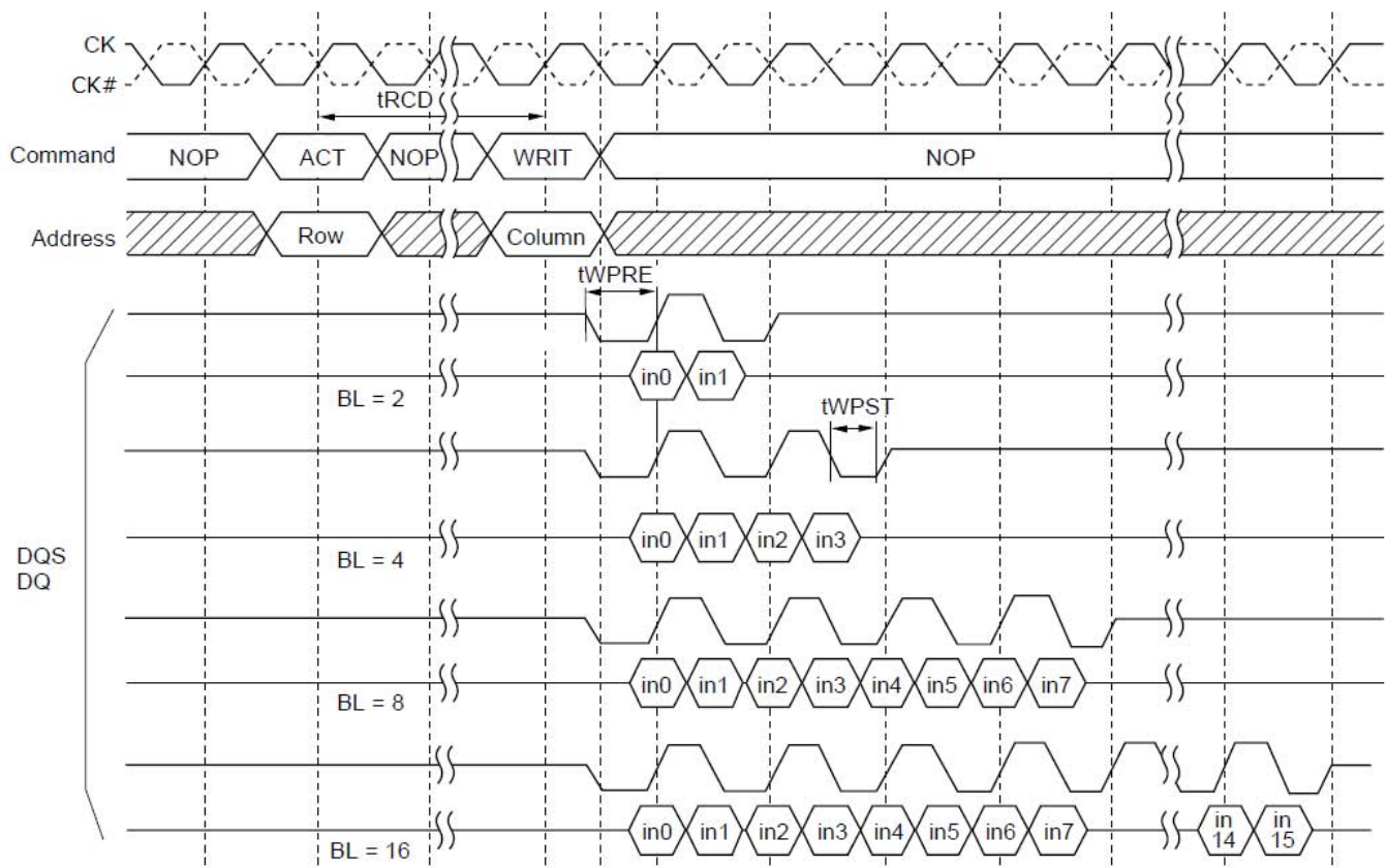
Figure 4.6 Write Operation
