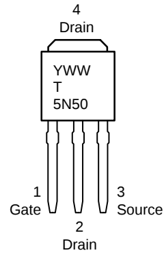
CASE 369 DPAK (Straight Lead) STYLE 2
