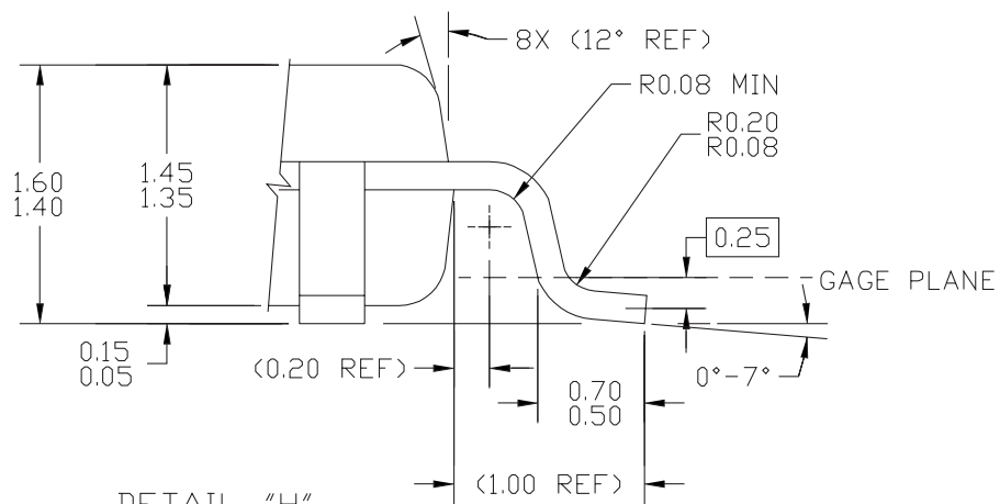
DETAIL "H"
