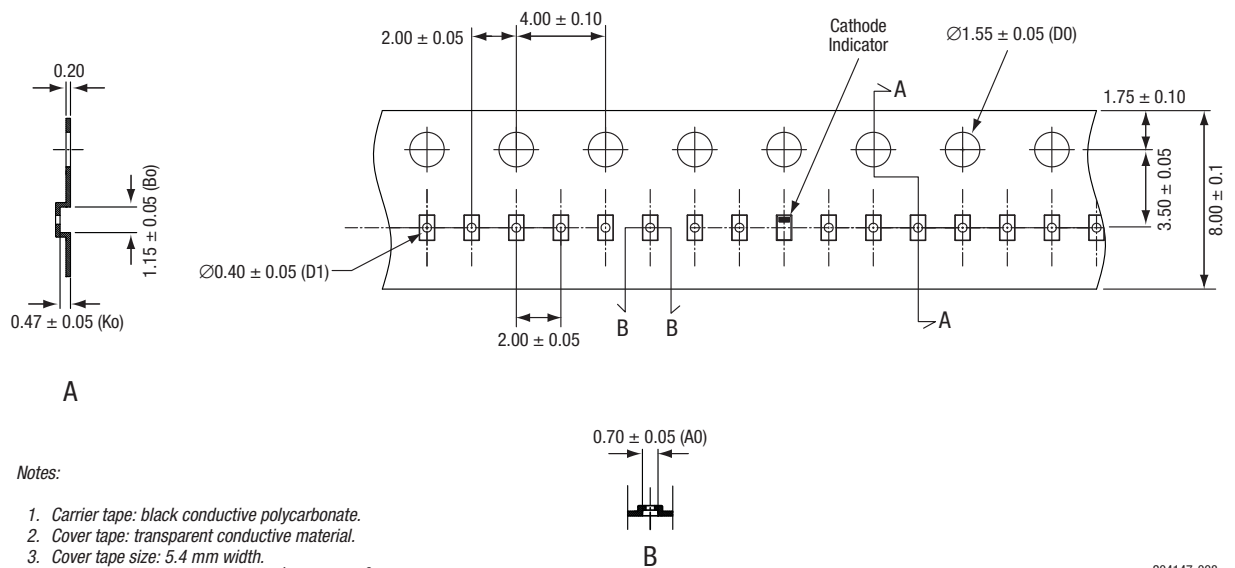
Figure 8. SOD-882 Tape and Reel Drawing
