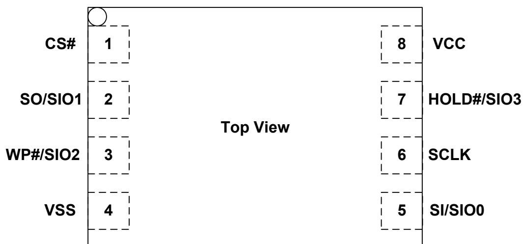
Figure 1-6. Pin Assignments
