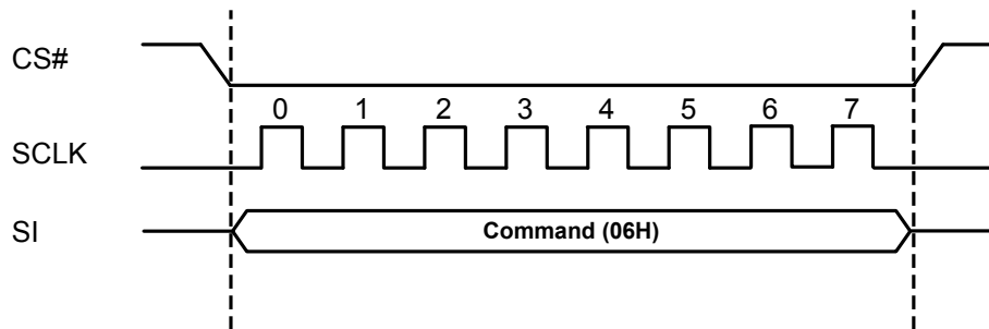
Figure 3-1. Write Enable (06H) Sequence Diagram
