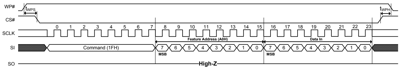
Figure 15-4. WP# Timing
