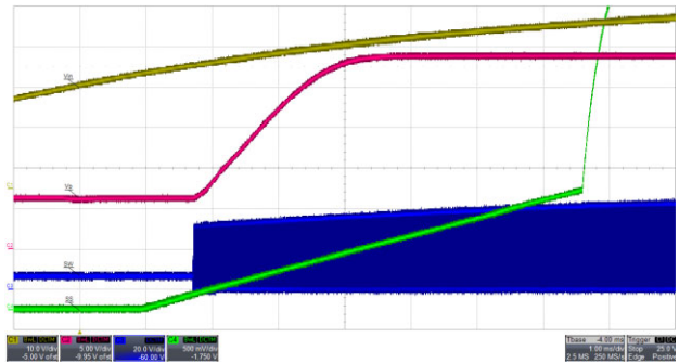
Figure 23. System Startup with 25% Pre-bias
