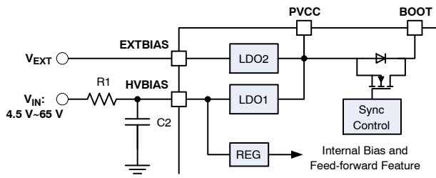
Figure 40. LDO Block Diagram
