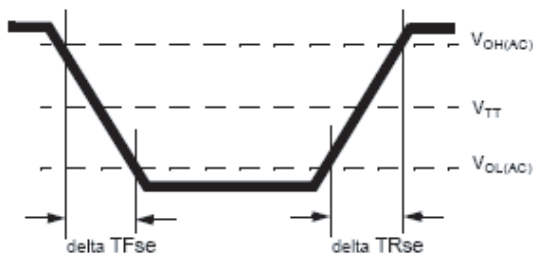
Single-ended Output Slew Rate definition
