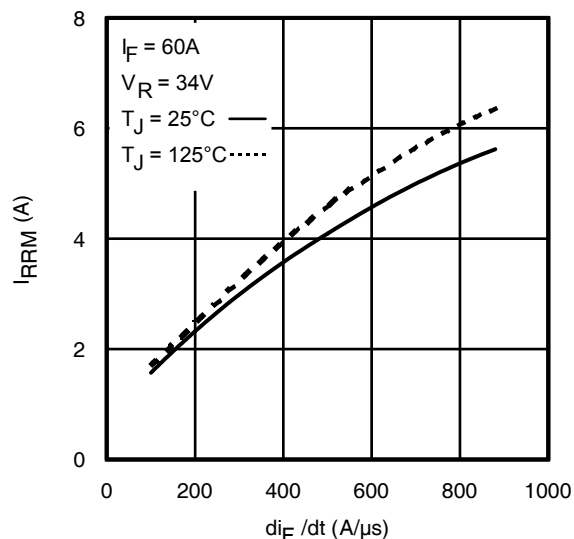
Fig. 19 - Typical Recovery Current vs. di/dt
