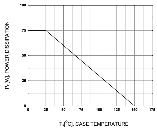
Figure 16. Power Derating
