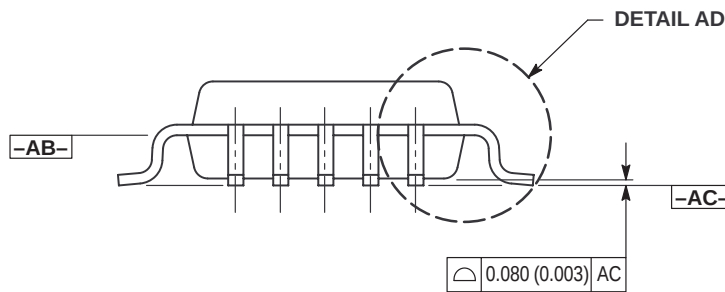
DETAIL AD
