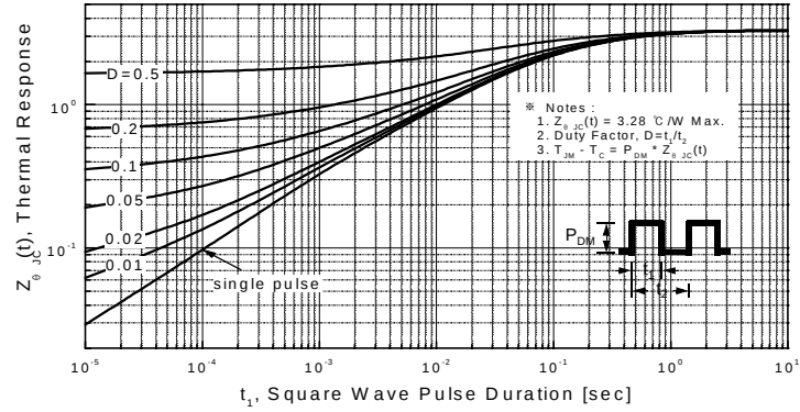
Figure 11-1. Transient Thermal Response Curve for IRF610B
