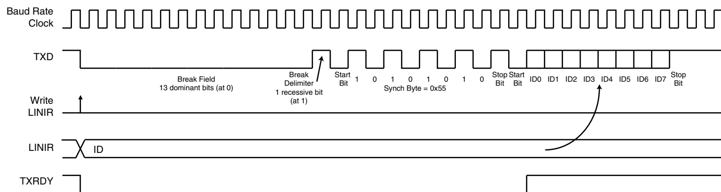
Figure 19-21. Header Transmission
