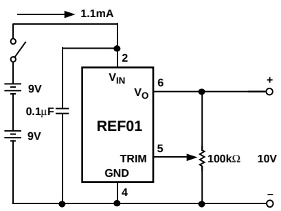
Figure 15. Precision Calibration Standard
