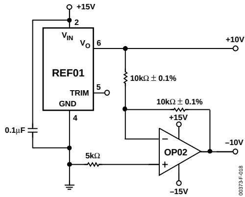
Figure 18. \pm 10\text{ V} Reference
