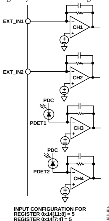
Figure 15. PD1 to PD4 Connection
