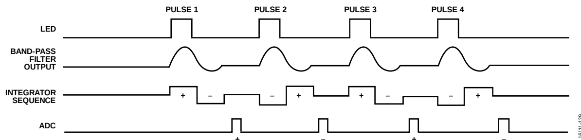
Figure 32. Diagram of Integrator Chopping Sequence
