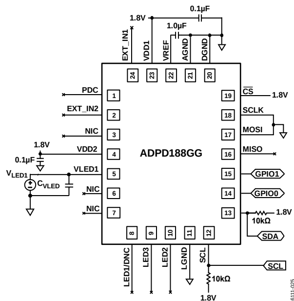
Figure 25. I 2 C Mode Connection Diagram
