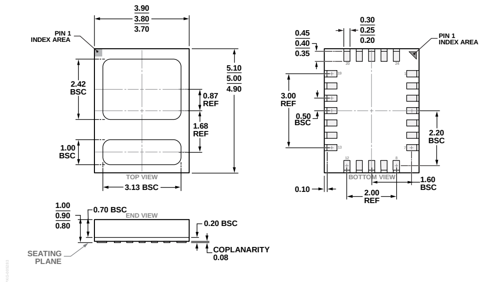
Figure 41. 24-Terminal Chip Array Small Outline No Lead Cavity [LGA_CAV] 3.80 mm × 5.00 mm Body and 0.9 mm Package Height (CE-24-1)
