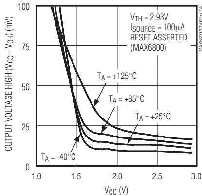
RESET ( V_{OH} ) vs. SUPPLY VOLTAGE
