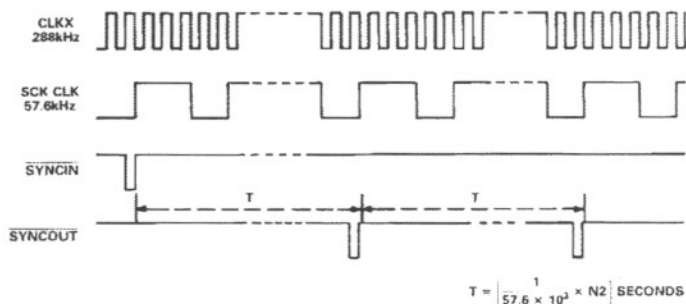
Figure 18. AD7341/AD7371 Timing Waveforms
