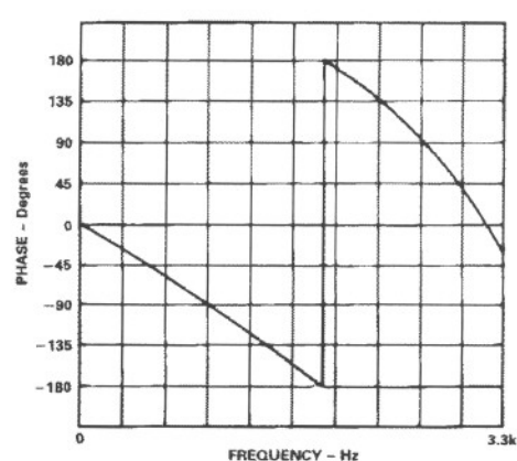
Figure 4. AD7341 Phase Response
