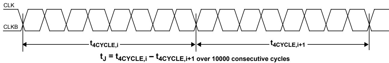
Figure 10. Short-term Jitter
