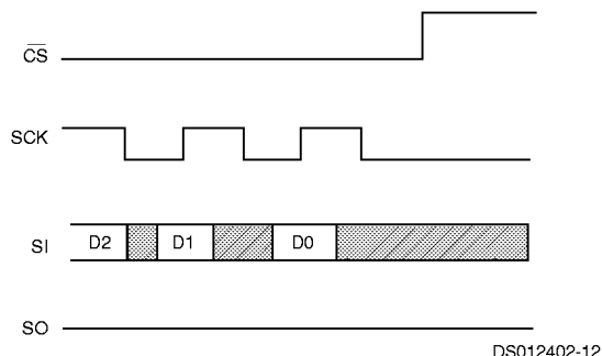
FIGURE 10. Write Sequence
