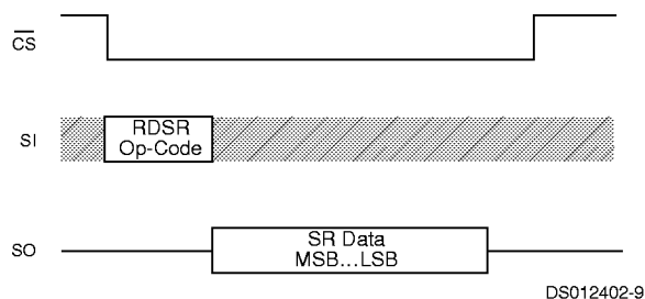
FIGURE 7. Read Status
