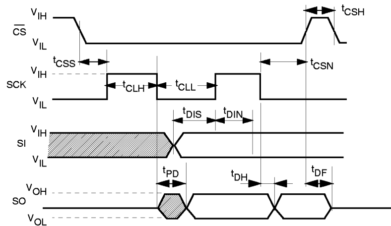
AC Test Conditions (Continued) FIGURE 1. Synchronous Data Timing Diagram
