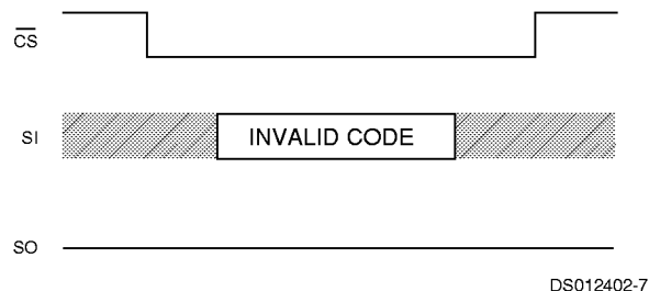
FIGURE 5. Invalid Op-Code
