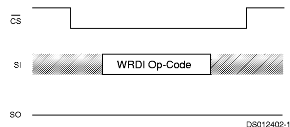
FIGURE 9. Write Disable
