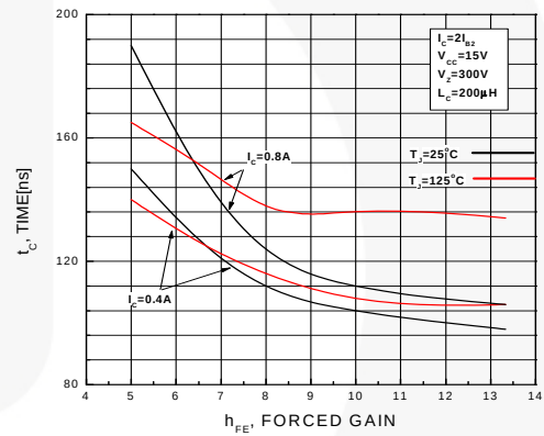
Figure 22. Inductive Switching Time, t_c
