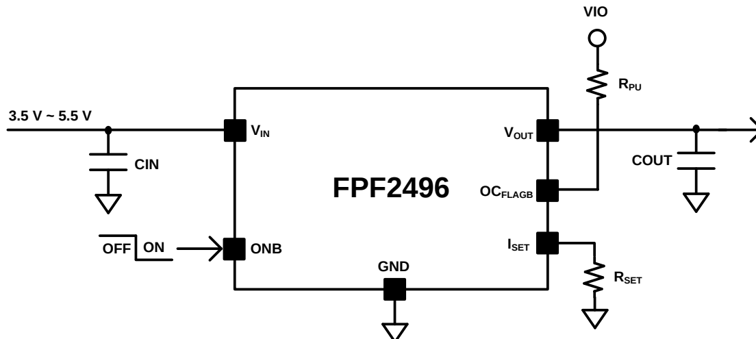
Figure 1. Typical Application
